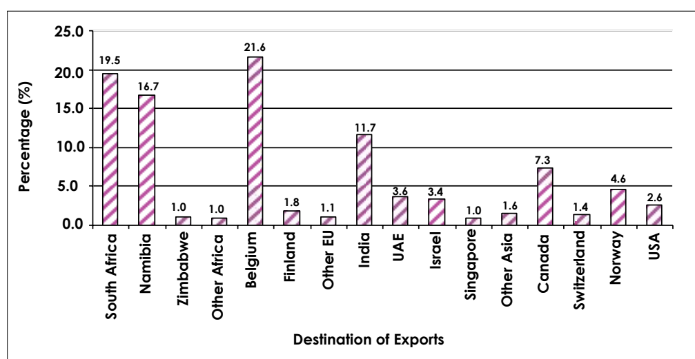
Chart 3.2: Exports by Major Trading Partners– December 2015
